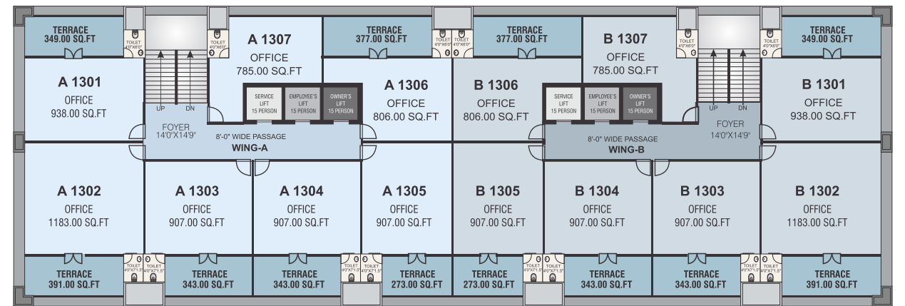
13 th Floor Plan
