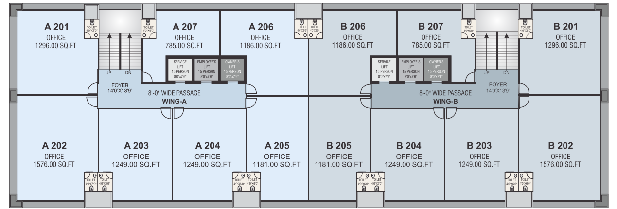
2 nd to 12 th Floor Plan
